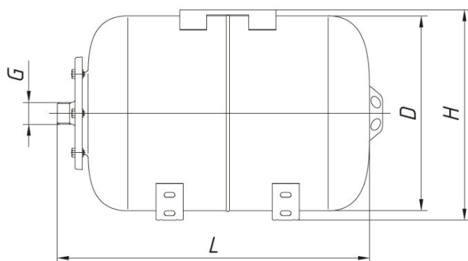
BASE 19 - 100 HOR
